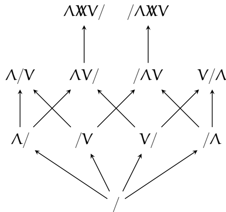
Figure 5: The eleven members of D_2 = [D_1 \rightarrow 3]
