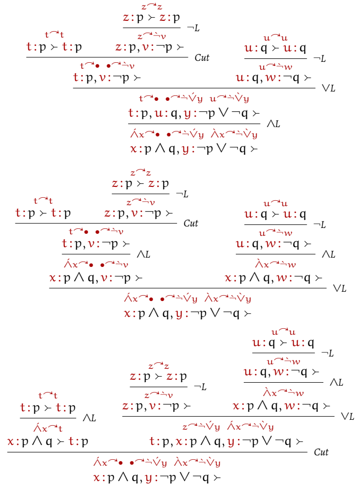
Figure 3: Three derivations with the term \hat{\lambda}x \rightarrow \bullet \rightarrow \dot{\vee}y \ \hat{\lambda}x \rightarrow \dot{\vee}y
